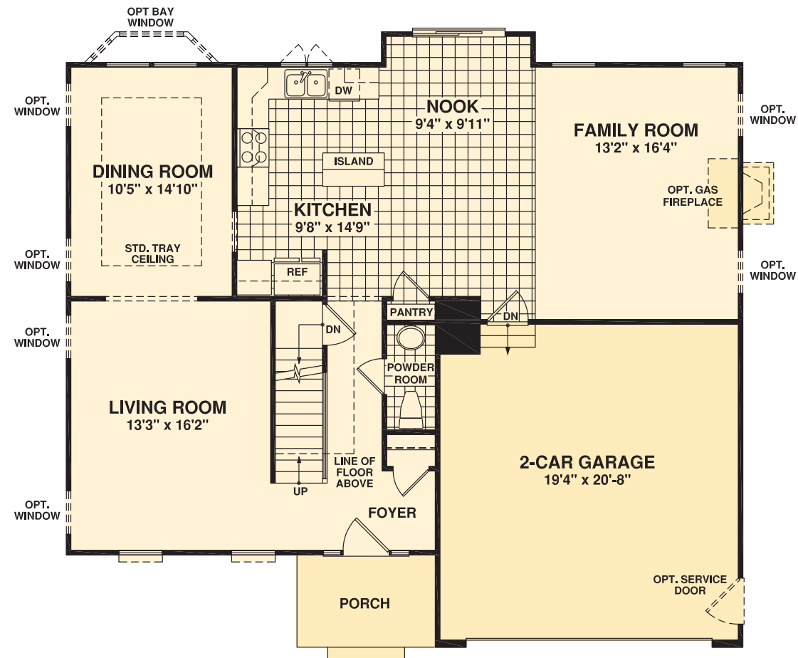
FIRST FLOOR PLAN w/ ELEV. #101 & #102
