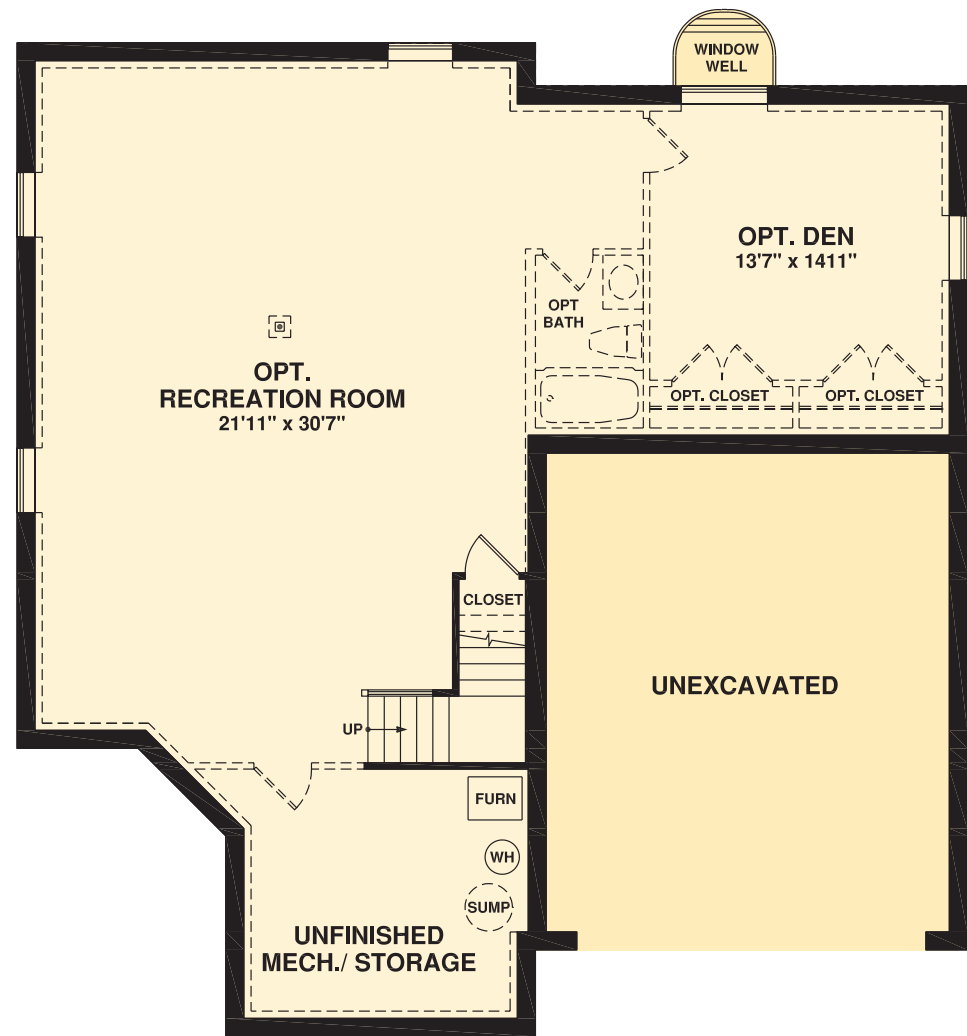
PARTIAL BASEMENT w/ OPT. WALKOUT CONDITION
