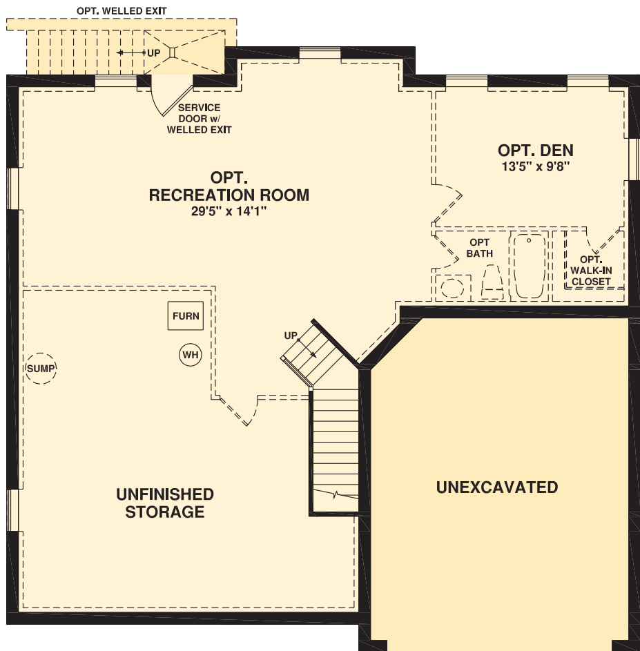
BASEMENT FLOOR PLAN w/ ELEV. 101, 102 & 103
