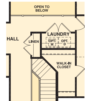
PARTIAL SECOND FLOOR w/ OPT. LAUNDRY ROOM
