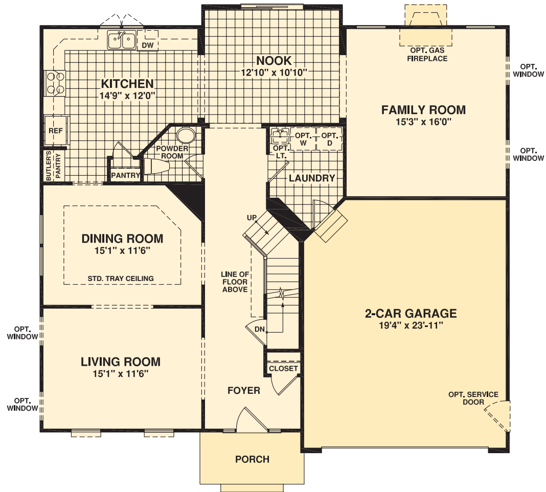
FIRST FLOOR PLAN w/ ELEV. #101 & #102
