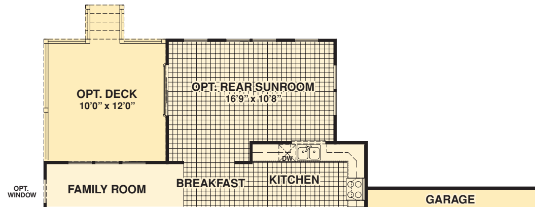
PARTIAL FIRST FLOOR w/ OPT. REAR SUNROOM
