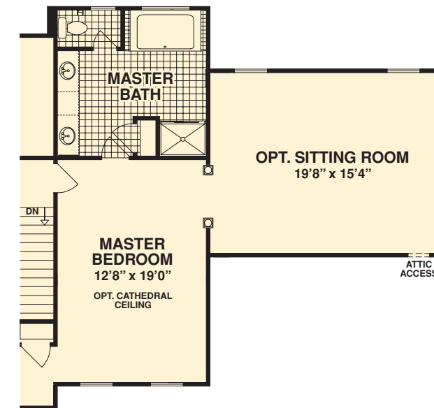
PARTIAL SECOND FLOOR PLAN w/ OPT. SITTING ROOM
